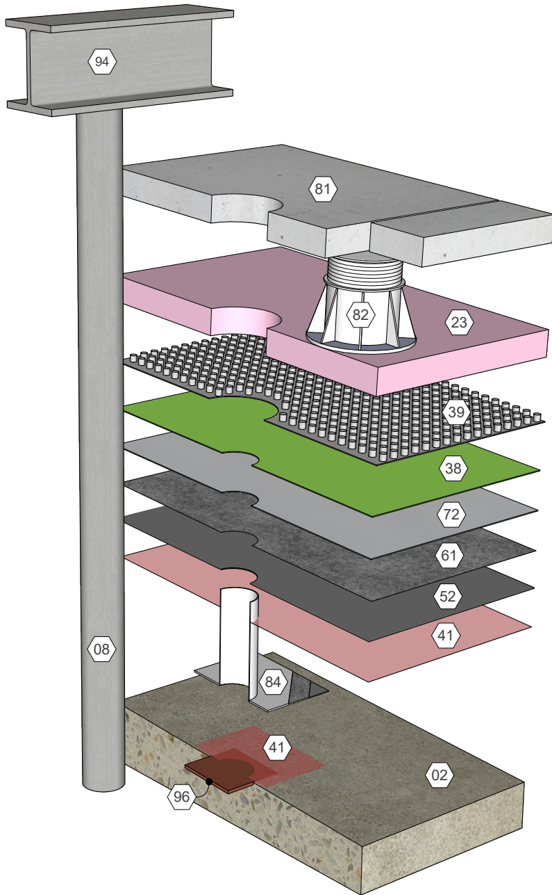
AlphaGuard® BIO Equipment Support Stand Leg Detail, Direct to Concrete Detail 10112
