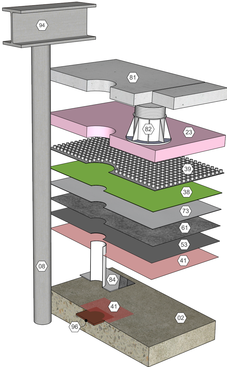
AlphaGuard® PUMA Equipment Support Stand Leg Detail, Direct to Concrete Detail 10113
