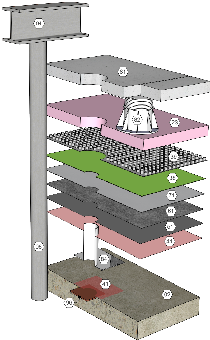
AlphaGuard® MT/MTS Plus Equipment Support Stand Leg Detail, Direct to Concrete Detail 10111
